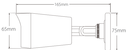
1080P Analog Camera
